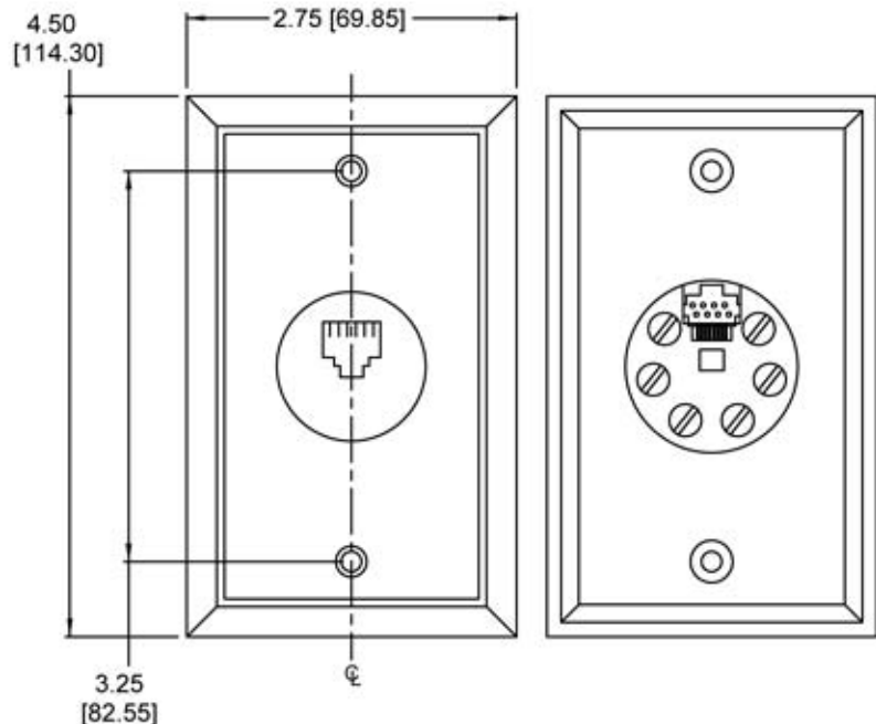
WIRING CONNECTIONS REAR VIEW
