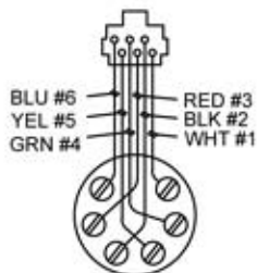
WIRING CONNECTIONS REAR VIEW
